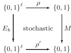
Fig. 8. A formulation of linear cryptanalysis as a stochastic commutative diagram attack. Here \rho and \rho' are linear maps
