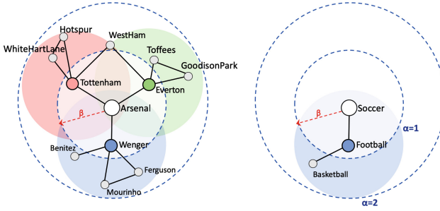
Fig. 1. Schematic of two \alpha -depth \beta -cut ego networks.
