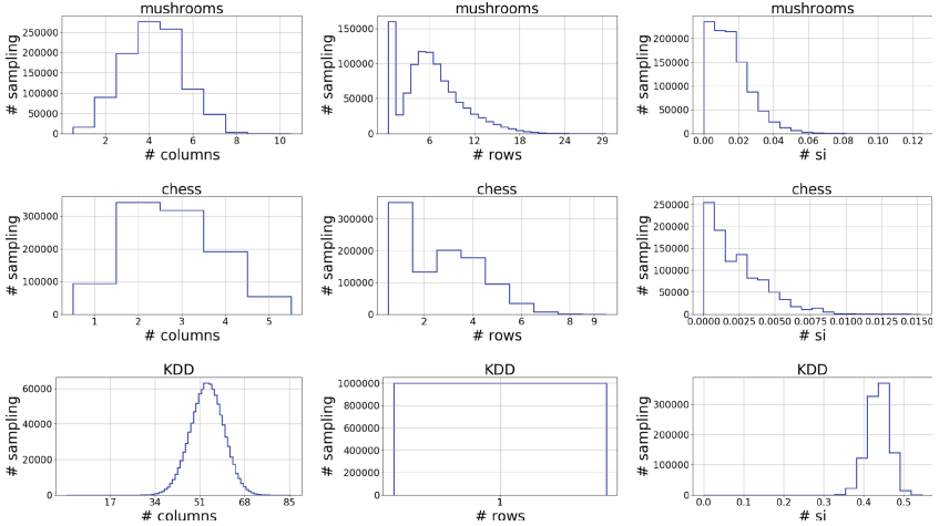
Fig. 2. Distributions of the sampled patterns w.r.t. # rows, # columns and SI.
