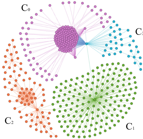
Fig. 3. The communities detected from the equality set containing the term http://dbpedia.org/resource/Barack.Obama using the Louvain algorithm. The 4 detected communities are distinguished by their nodes' color. The full figure is available at https://github.com/raadjoe/LOD-Community-Detection/blob/master/Communities-Graph-Obama.svg . (Color figure online)
