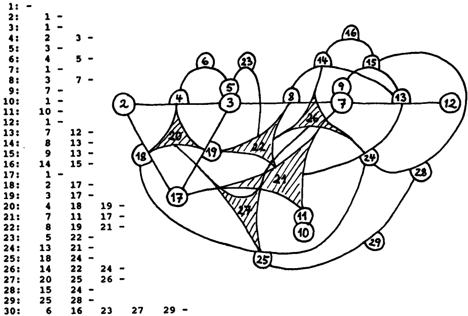
Fig. 6. List of upper covers in the concept lattice "Rohbau" and geometric representation derived from it
