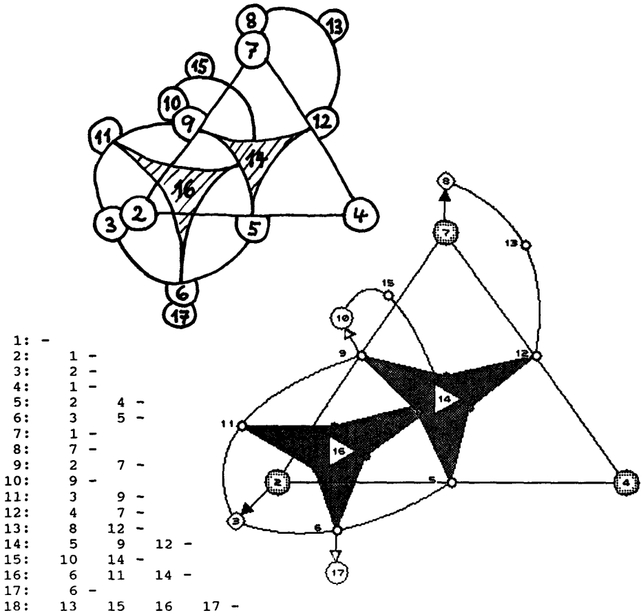
Fig. 3. List of upper covers and geometric representations of the lattice in Fig. 2
