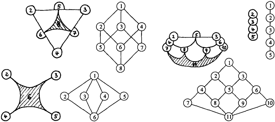
Fig. 4. Linediagrams and geometric representations of lattices
