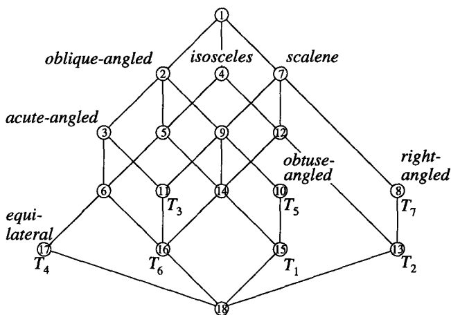
Fig. 2. Concept lattice of the context in Fig. 1
