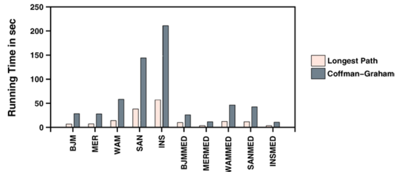
Fig. 9. Running time for AT&T graphs
