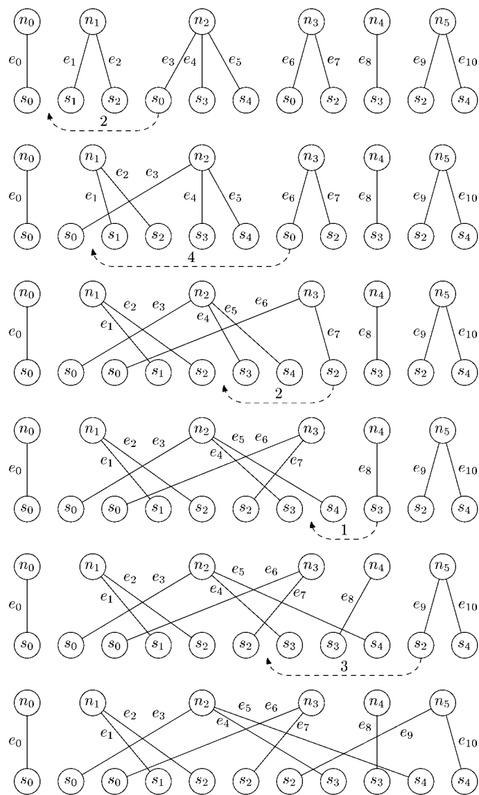
Fig. 3. Counting crossings via insertion sort
