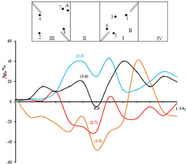
Fig. 9. Typical anisotropy registered in electrical resistivity measured for different positions of pick-up electrode pairs in granite sample. Scheme of four (I-IV) sample facets with the introduced stress concentrators, pick-up electrodes: 1, 2, 3, 4, 5, 6, 7, and feeding electrodes A, B are shown above the plot.
