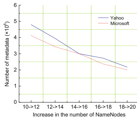
Fig. 11 Migration overhead
