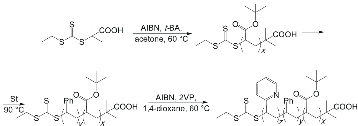
Fig. 2. Synthetic routes of block copolymers preparation.
