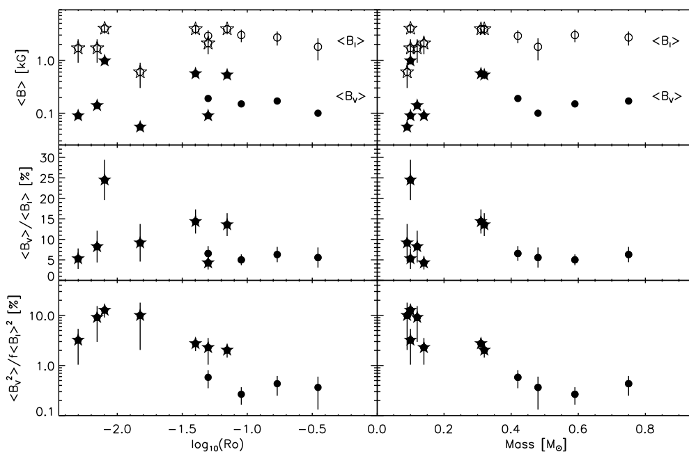
Figure 24: Measurements of M dwarf magnetic fields from Stokes I and Stokes V. Top panel: Average magnetic field – Open symbols: measurements from Stokes I; Filled symbols: measurements from Stokes V. Center panel: Ratio between Stokes V and Stokes I measurements. Bottom panel: Ratio between magnetic energies detected in Stokes V and Stokes I. Circles show objects more massive than 0.4 M_{\odot} , stars show objects less massive than that.
