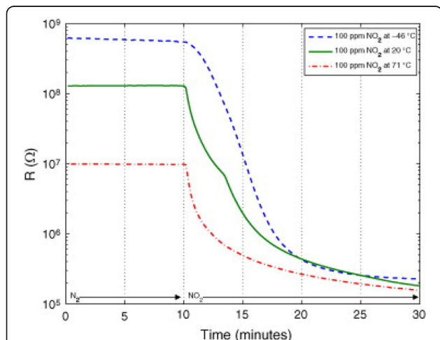
Fig. 15 Response of sensors to 30-min 100 ppm NO 2 exposure (reprinted with permission from Reference Shu et al. 2010). © 2010 Elsevier
