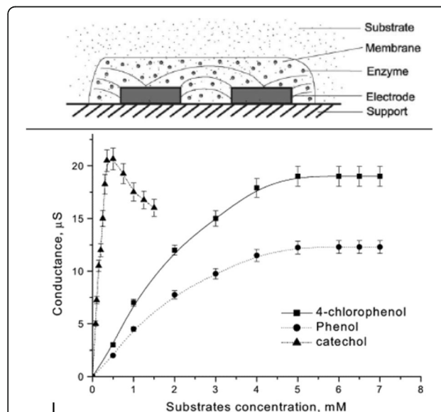
Fig. 16 (Upper) Schematic representation of conductometric biosensor; (below) calibration curves of conductometric tyrosinase biosensor for 4-chlorophenol, phenol, and catechol. (Reprinted with permission from Reference Anh et al. 2004). © 2004 Elsevier
