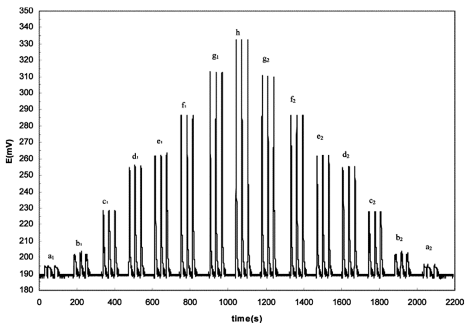
Fig. 3 Potentiometric peaks for three repetitive measurements of different Pb 2+ ion concentrations. (Reprinted with permission from Reference Karami et al. 2003). © 2003 Elsevier
