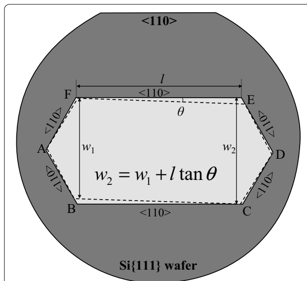
Fig. 3 Effect of misalignment on the size of the structure fabricated using wet anisotropic etching on Si{111} wafer. \theta is the misalignment angle of mask edge from (110) crystallographic direction. Dashed lines indicate the edges of original hexagonal shape mask pattern
