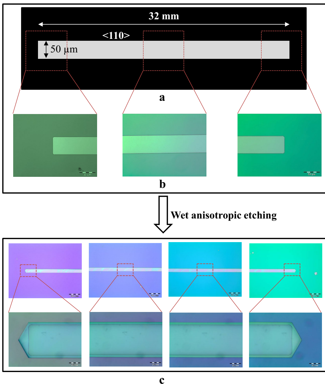
Fig. 6 A 50 μm wide and 32 mm long rectangular shape mask opening with longer edge aligned along the \langle 110 \rangle direction on \{111\} wafer surface to test the accuracy of proposed method: a schematic diagram, b optical image of the mask pattern after oxide etching, c etched profile with zoomed-in images of different portions. Pre-etched patterns are used as reference for the precise alignment of the mask edges along \langle 110 \rangle direction. The undercutting at the mask edges takes place due to finite etch rate of \{111\} plane and the uniform undercutting indicates the accurate alignment of mask edges along \langle 110 \rangle direction
