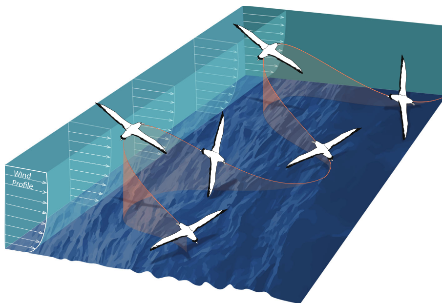
Fig. 1 Schematic diagram showing an albatross flying in an across-wind direction using an S-shaped dynamic soaring maneuver (redrawn from [13]). The bird is shown soaring through a vertical profile of mean wind velocity. The bird extracts energy from the wind by climbing headed upwind and descending headed downwind. Significant waves are typically observed in the Southern Ocean. Wind-wave interactions cause a more complicated instantaneous wind field than that plotted here. Albatrosses appear to efficiently exploit the instantaneous in-situ winds and waves in dynamic soaring
