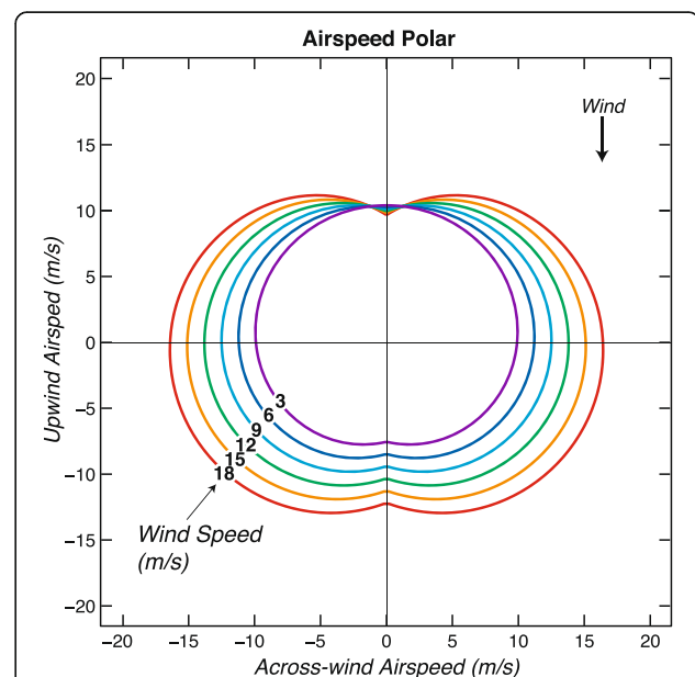
Fig. 5 Polar diagram showing modeled airspeed averaged across the sexes as a function of wind speed and relative wind direction for six different wind speeds as calculated with a linear model (Eq. 4). The average wind speed is 9.0 m/s so the airspeed curve for this wind speed (light blue) is representative of average airspeeds. Across-wind components of modeled air velocity are plotted against upwind components of modeled air velocity
