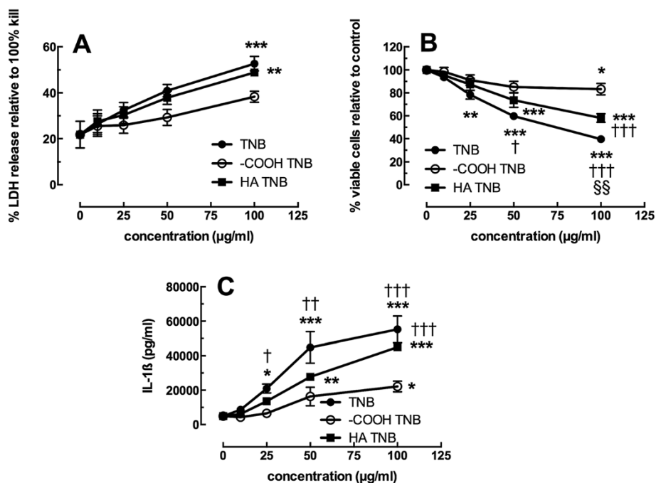
Figure 12 Viability and IL-1 \beta release following 24-h exposure to TiO 2 nanobelts in transformed human THP-1 cell line. A) Mean \pm SEM percent LDH release relative to total cell lysis. B) Mean \pm SEM percent viable cells relative to no particle control. C) Mean \pm SEM IL-1 \beta release. Asterisks indicate significance at *** P < 0.001, ** P < 0.01, or * P < 0.05 compared to no particle 0 \mu g/ml condition. Daggers indicate significance at ††† P < 0.001, †† P < 0.01 or † P < 0.05 compared to the TiO 2 -COOH nanobelt (TNB COOH) at the same concentration. Symbols §§ indicate significance at P < 0.01 compared to the humic acid TiO 2 nanobelt (TNB HA) condition at the same concentration.
