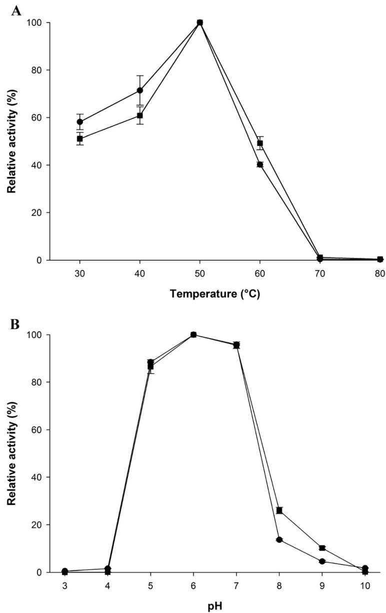
Figure 2 Effect of temperature (A) and pH (B) on recombinant \beta -mannanase activity. Extracellular (—●—) and intracellular (—■—) enzymes were used for these experiment, and results are expressed as relative activity. (100% relative activity of extracellular and intracellular enzymes were 37.10 and 515.00 U per ml, respectively).
