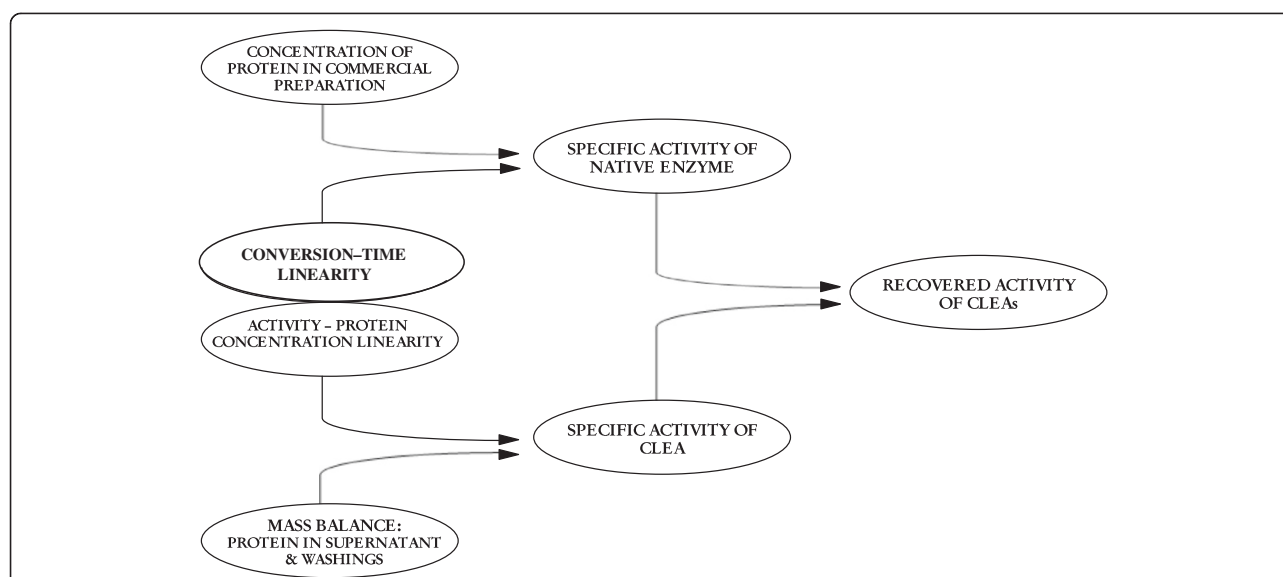
Figure 1 Scheme of calculation of recovered enzymatic activity in CLEAs.
