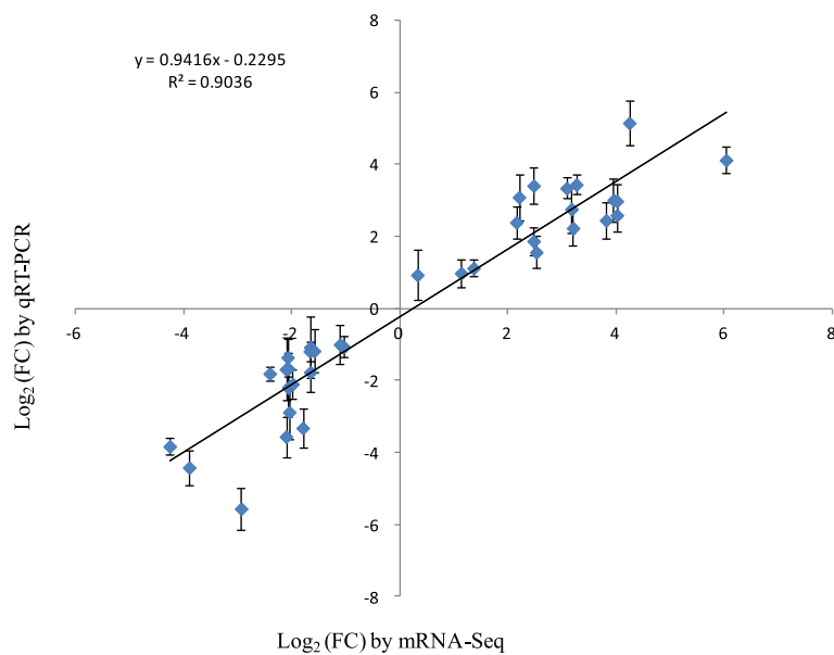
Figure 7 Comparison of the \log_2(\text{FC}) of 18 selected transcripts using RNA-Seq and qRT-PCR.
