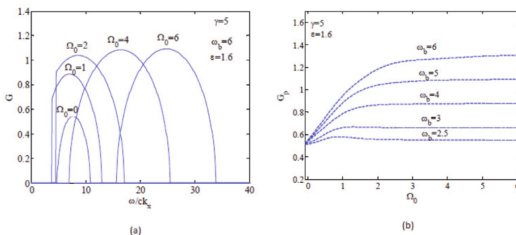
Fig. 1. (a) Growth rate G as function of the normalized radiation frequency \omega/ck_x for different values of normalized axial magnetic field \Omega_0 = 0, 1, 2, 4 , and 6 . (b) Peak growth rate G_p as function of the normalized axial magnetic field \Omega_0 for different values of normalized electron beam frequencies \omega_b = 2.5, 3, 4, 5 , and 6 . Here, self-fields are ignored.
