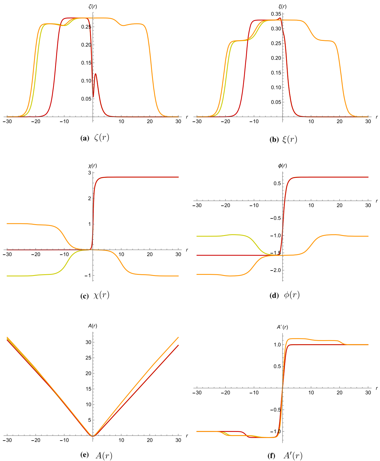
Fig. 8 Profiles of scalar fields ( \zeta, \xi, \chi, \phi ) and the warped factor A for SO(8)/U(3) Janus together with SO(8)/G_2 and G_2/G_2 solutions that flow to the U(3) critical point as functions of the radial coordinate r
