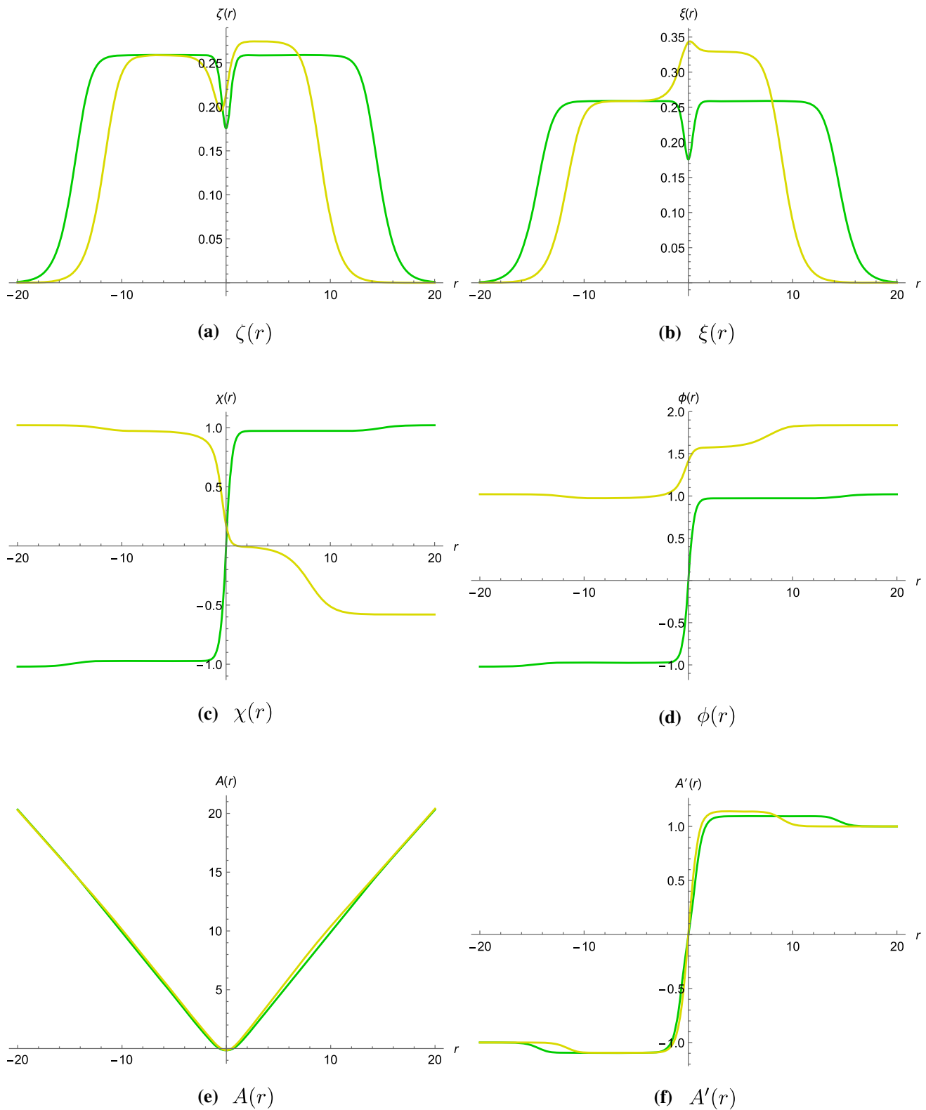
Fig. 4 Profiles of scalar fields ( \zeta, \xi, \chi, \phi ) and the warped factor A for G_2/G_2 and G_2/U(3) Janus solutions as functions of the radial coordinate r are shown by green and yellow lines, respectively
