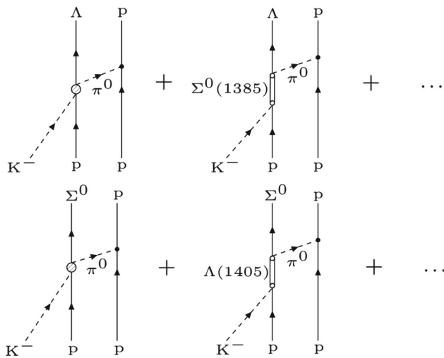
Fig. 5 The tree level (left) and the leading order (right) diagrams of the processes K^-(pp) \rightarrow \Lambda p (top) and K^-(pp) \rightarrow \Sigma^0 p (bottom), according to the meson exchange model
