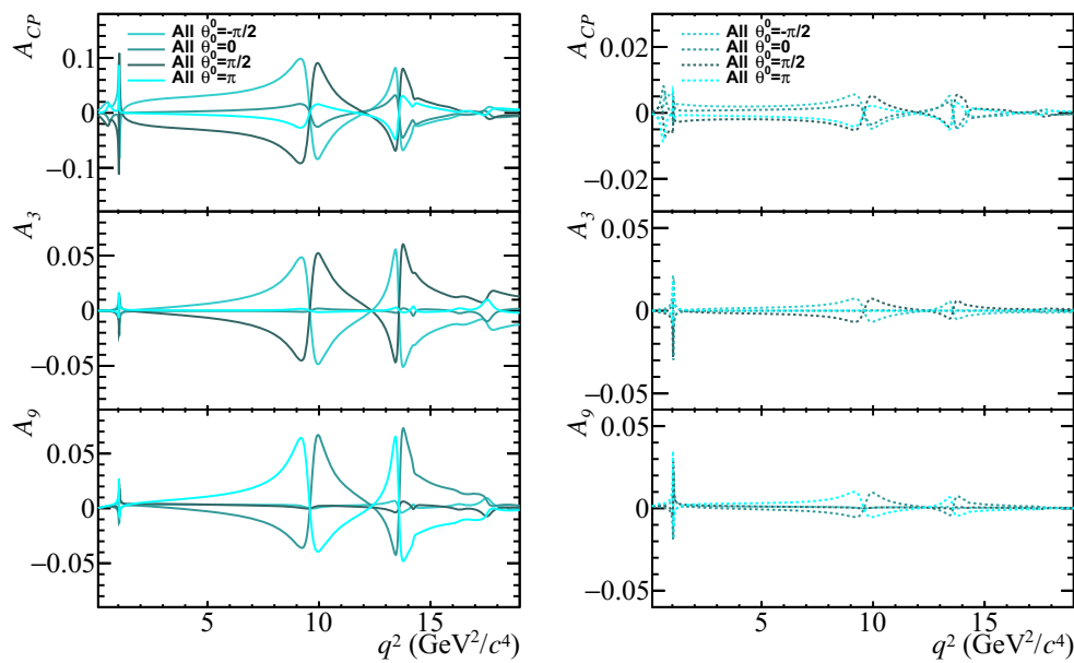
Fig. 4 Distribution of observables A_{CP} , A_3 and A_9 as a function of q^2 , for \theta_j^0 of all resonances set to -\pi/2, 0, \pi/2 and \pi . Two new physics models are considered, one with C_9^{NP} = -1.0 - 1.0i (left), and one with C_7^{NP} = -0.03i, C_9^{NP} = -1.0 (right)
