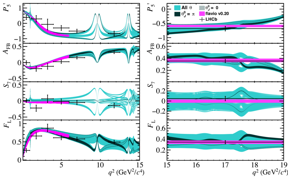
Fig. 3 Distributions of the angular observables P'_5 , A_{FB} , S_7 , and F_L as a function of q^2 for regions below (left) and above (right) the open charm threshold (cyan). Specific choices are highlighted for \theta_j^0 = 0 (hatched band) and \theta_j^0 = \pi (dark band). The measured values of the
