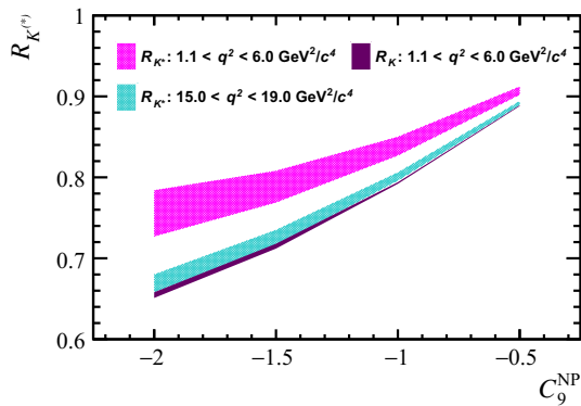
Fig. 6 Predictions of R_{K^*} at large recoil (hatched magenta) and low recoil (hatched cyan), and R_K at large recoil (solid burgundy) for different values of C_9^{\text{NP}} . The R_K values at low recoil are identical to those at large recoil and thus not shown. The interval for R_{K^*} is determined using the model described in Sect. 2, considering the full variation of the unknown phases \theta_j^0 . In contrast the 68% confidence interval of the R_K prediction is obtained using the measured non-local contributions in B^- \rightarrow K^- \mu^+ \mu^- decays [20]
