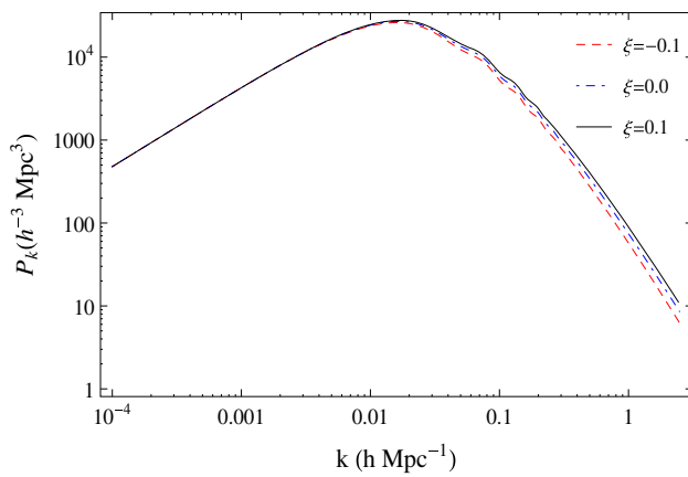
Fig. 2 The matter power spectrum for \xi = -0.1 (dashed), 0 (dash-dotted), 0.1 (solid)
