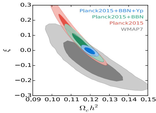
Fig. 3 Marginalized two-dimensional contours in the \xi - \Omega_c h^2 plane with 68 and 95% confidence level in the extended \Lambda CDM model with BBN consistency, derived from the data of Planck 2015 + JLA + BAO (green) and Planck 2015 + JLA + BAO + Y_p (blue). The red and gray contours correspond to Y_p = 0.24 , derived from Planck 2015 + JLA + BAO and from WMAP7 + H_0 + BAO [22], respectively
