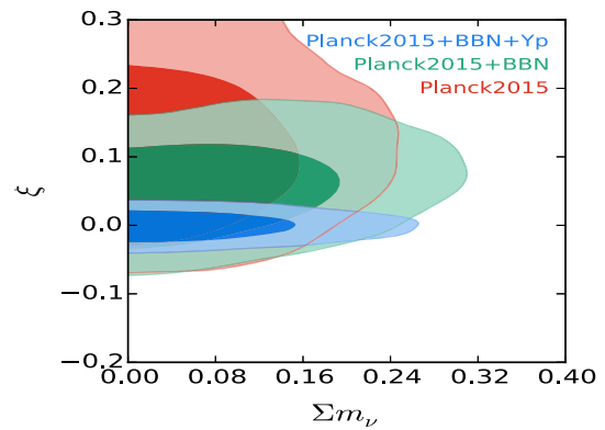
Fig. 5 Marginalized two-dimensional contours in the \xi - \Sigma m_\nu plane with 68 and 95% confidence level in the extended \Lambda CDM model with BBN consistency, derived from the data of Planck 2015 + JLA + BAO (green) and Planck 2015 + JLA + BAO + Y_p (blue). The red contours correspond to Y_p = 0.24 , derived from Planck 2015 + JLA + BAO
