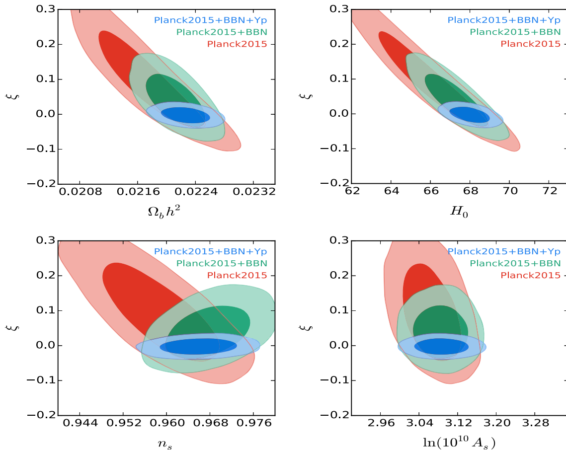
Fig. 4 Marginalized two-dimensional contours in \xi - \Omega_b h^2 (top-left), \xi - H_0 (top-right), \xi - n_s (bottom-left) and \xi - A_s (bottom-right), with 68 and 95% confidence level in the extended \Lambda CDM model with
