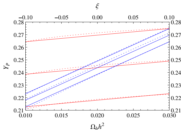
Fig. 1 BBN-predicted curves for Y_p in \Omega_b h^2 (red) and \xi (blue). From bottom to top, the red curves correspond to \xi = -0.1, 0, -0.1 , while the blue curves correspond to \Omega_b h^2 = 0.01, 0.02, 0.03 . The dotted curves are the BBN-predicted results, while the solid curves are our fits
