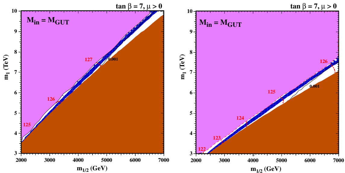
Fig. 2 Examples of (m_{1/2}, m_1) planes for M_{in} = M_{GUT} and \tan \beta = 7 when both Higgs 5-plets are twisted. In the left panel, all the modular weights \alpha_i = \beta_i = 0 , corresponding to A_{t,b} = m_1 , A_\lambda = 2m_{3/2} , A_{\lambda'} = 0 , B_H = 2m_1 , and B_\Sigma = 0 . In the right panel, the modular weights are chosen to be \alpha_{t,b} = 1 , \alpha_\lambda = 2 , \alpha_{\lambda'} = 0 , \beta_H = 2 and \beta_\Sigma = 0 , corresponding to A_0 = B_0 = 0 . The shadings and contour
