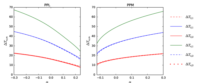
Fig. 1 Time delays between different relativistic images for Sgr A*. \Delta T_{n,m} are represented in units of 2GM_\bullet/c^3 \approx 42.45 s. The left panel shows the time delays for the case of PPL ( 4\alpha < 1 ) and the right one is for PPM ( 8\alpha > -1 )
