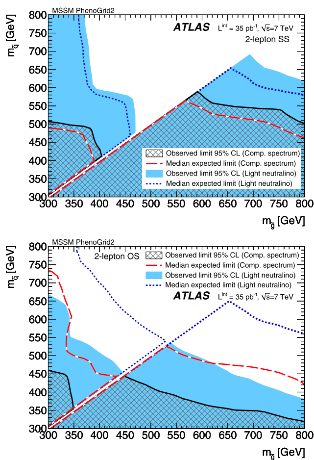
Fig. 3 Expected and observed 95% C.L. exclusion limits in the ( m_{\tilde{g}}, m_{\tilde{q}} ) plane for the specific MSSM models described in the text. The upper panel is for the SS analysis, the lower panel for the OS analysis
