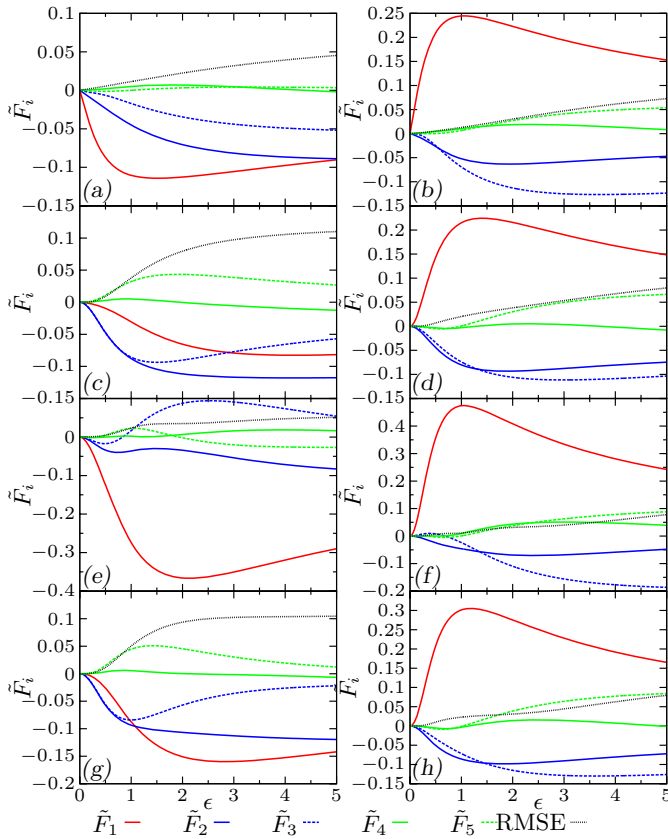
Fig. 9. Amplitudes of the Fourier decomposition (36) for dots (left column) and holes (right column) with Y = Y_{\text{const}} . (a,b) f_{\text{const}} , (c,d) f_{\cos \theta} , (e,f) f_{\text{spec}} , (g,h) f_{\text{skew}} .
