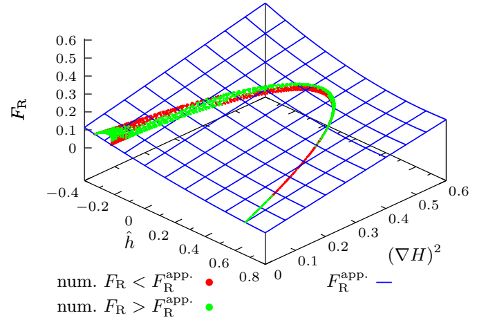
Fig. 6. Numerically determined redeposition F_R plotted versus relative height \hat{h} and squared slope (\nabla H)^2 (here for hexagonal dots, \epsilon = 0.25 , f_{\text{skew}} , Y_{\text{const}} ). A least square fit determines the coefficients of the approximation F_R^{\text{app.}} . For the sake of visibility, the numerical data for F_R below and above F_R^{\text{app.}} is indicated by red and green points, respectively.
