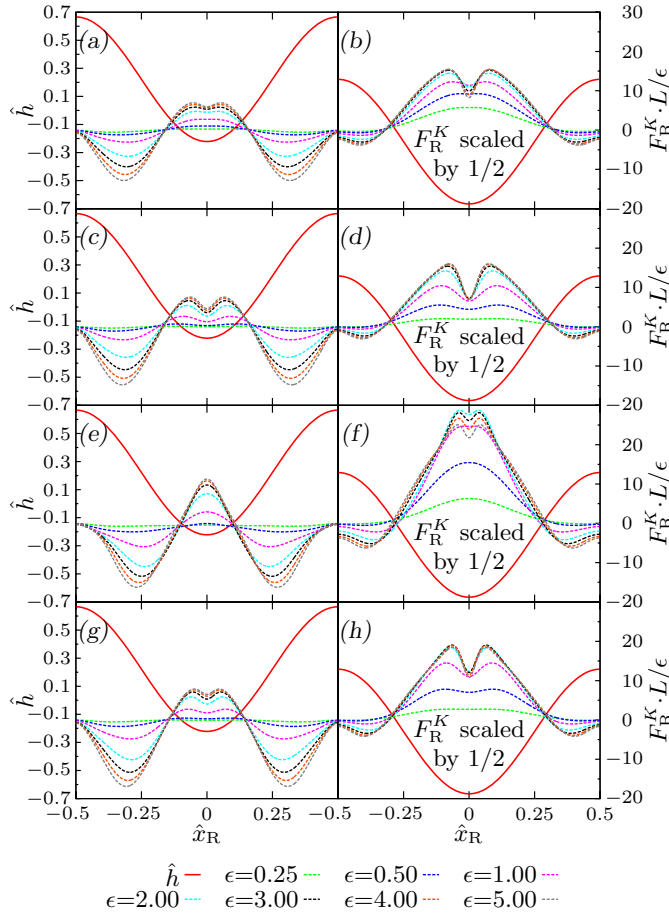
Fig. 12. Cross-sectional plots of the curvature-dependent portion F_R^K for dots (left column) and holes (right column). (a,b) f_{\text{const}} , (c,d) f_{\cos\theta} , (e,f) f_{\text{spec}} , (g,h) f_{\text{skew}} .
