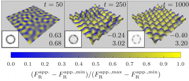
Fig. 19. Evolution of the approximated equation (52) with constant parameters according to (49). The values in the lower right of the pictures are \beta F_R^{\text{app.,min}} and \beta F_R^{\text{app.,max}} , i.e. maximum and minimum of the color-coded approximated redeposition.
