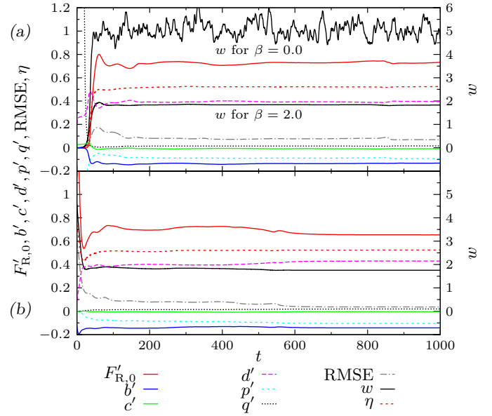
Fig. 18. (a) Temporal evolution of the fit coefficients for the simulation depicted in Figure 16a. Additionally, the roughness w of Figure 16b is shown. (b) Coefficient curves for the evolution of Figure 16c.
