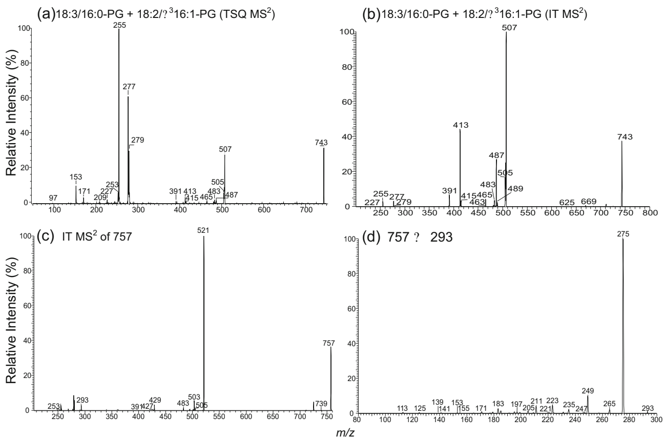
Figure 3. The product-ion spectrum of the ion at m/z 743 obtained with (a) a TSQ, and (b) an IT instrument. Panel (c) is the IT MS 2 -spectrum of the ion at m/z 757, which may consist of a 18:3/ \Delta^3 16:1-PG structure. The presence of the hydroxylated 18:3-fatty acid substituent is consistent with the presence of a prominent ion at m/z 275, corresponding to loss of H 2 O from m/z 293, as shown in the MS 3 -spectrum of m/z 293 (757 → 293) (d).
