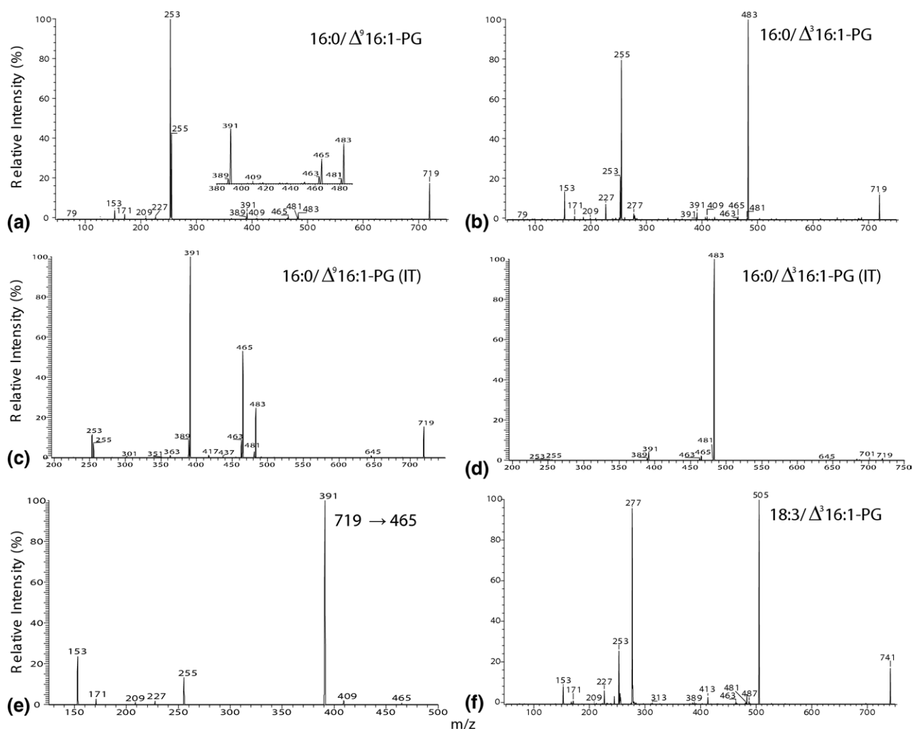
Figure 2. The TSQ product-ion spectra of (a) 16:0/ \Delta^9 16:1-PG, (b) 16:0/ \Delta^3 16:1-PG, and the corresponding IT MS 2 spectra of (c) 16:0/ \Delta^9 16:1-PG, (d) 16:0/ \Delta^3 16:1-PG. The MS 3 -spectrum of the ion at m/z 465 ( 719 \rightarrow 465 ) (e) illustrates that the ions at m/z 227, 171, and 153 that are characteristic ions of PG and the ion at m/z 391, which is a precursor ion of the carboxylate anion at m/z 255 arise from sequential fragmentation of m/z 465. Panel (f) is the product-ion spectrum of the ion at m/z 741, which is similar to the spectrum shown in (b), suggesting the presence of 18:3/ \Delta^3 16:1-PG, the major species found in the PG extract.
