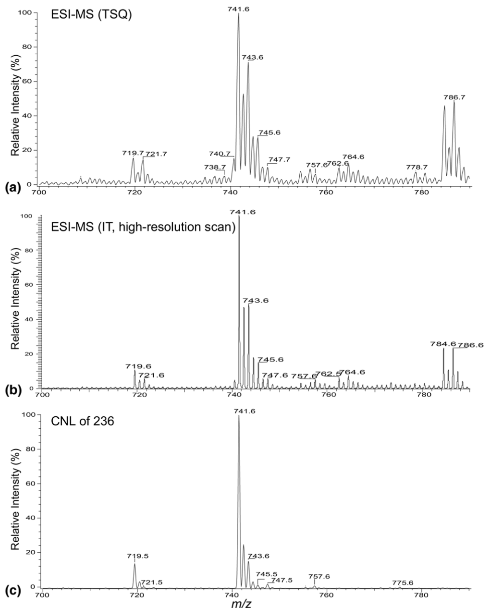
Figure 1. The full scan mass spectra of the lipid extract from plant chloroplasts obtained with (a) a tandem quadrupole, and (b) an IT instrument. Panel (c) shows the tandem mass spectrum of the same mixture acquired by CNL of 236, exhibiting the PG species that contain a 16:1-fatty acid substituent, mainly a \Delta^3 16:1-fatty acid substituent at sn -2 in the mixture.
