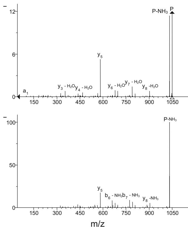
Figure 1. Comparison of the MS/MS spectrum of the singly protonated QLLPLLLK ion measured in the ion-trap mass spectrometer (bottom) with a spectrum measured in the triple quadrupole instrument at an intermediate collision energy (top). While the precursor peak is completely depleted in the ion-trap spectrum, a large fraction of it still remains in the triple quadrupole spectrum, as is evident from the different intensity scales (y axis).
