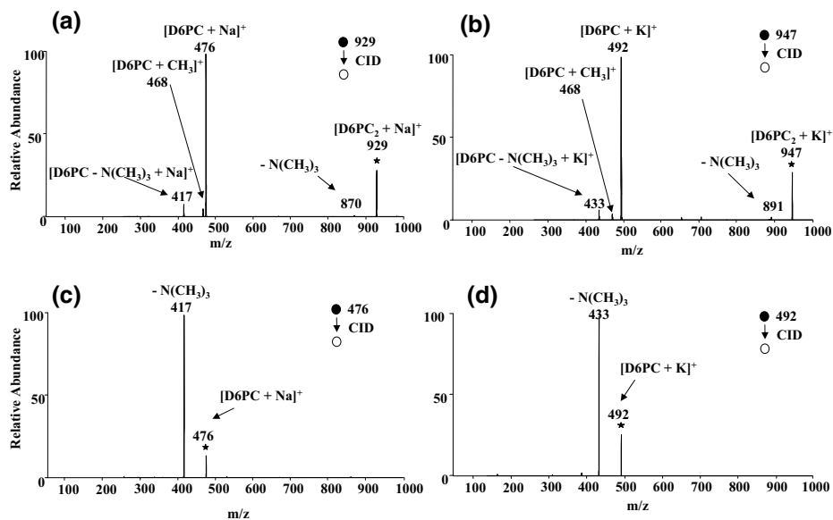
Figure 2. LCQ CID MS/MS of (a) [D6PC_2 + Na]^+ ; (b) [D6PC_2 + K]^+ ; (c) [D6PC + Na]^+ ; (d) [D6PC + K]^+ . The mass selected precursor ion is designated by an asterisk.
