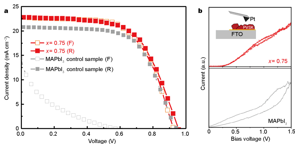
Figure 6 (a) J - V curves under different scan directions of perovskite solar cells based on \text{PbI}_2 \cdot (1-x)\text{FAI} \cdot x\text{MACl} , x=0.75 and \text{MAPbI}_3 ; (b) J - V curves under different scan directions performed on a single perovskite grain for both samples with c-AFM.
