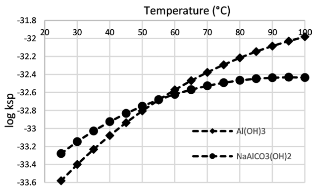
Fig. 2 a Aluminum speciation diagram of PLS, b Solubility product constant ( k_{sp} ) of aluminum hydroxide ( \text{Al}(\text{OH})_3 ) and dawsonite \text{NaAlCO}_3(\text{OH})_2 versus temperature. [where a=aqueous, a- aqueous anion, a+ aqueous cation]
