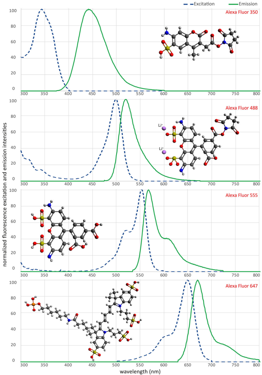
Fig. 7 Specific absorption and emission spectra of different fluorescent molecules [25]
