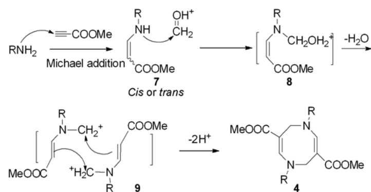
Scheme 2 Plausible mechanism of the acid-mediated MCR
