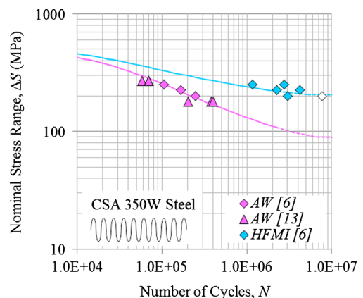
Fig. 14 Fracture mechanics analysis result for CSA 350W steel (CA loading)
