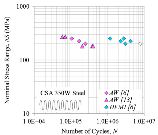
Fig. 4 CA results for CSA 350W steel from [6, 13]
