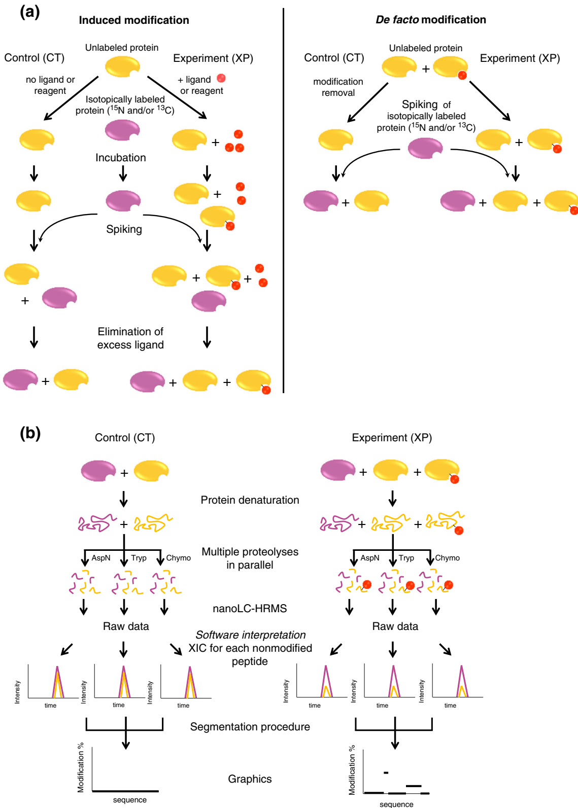
Figure 1. Quantification workflow. (a) Preparation of the samples and their controls for quantification of de facto or induced modifications. (b) Production of peptides and nanoLC-HRMS quantification of the nonmodified peptides
