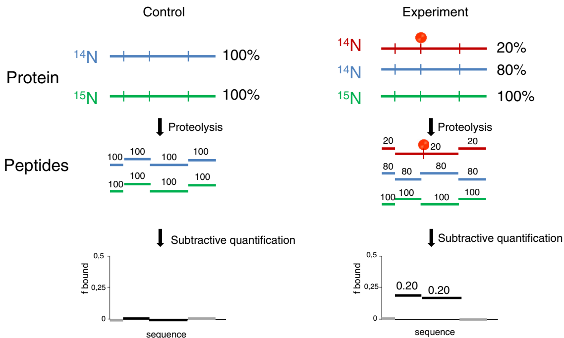
Figure 3. Bound fraction pattern caused by a missed cleavage caused by the modification. This scheme is valid for both N- and C-endoproteinases. Protein and peptides are represented in color with associated abundances. The corresponding f_{\text{bound}} s are calculated based on changes in nonmodified peptides and graphed at the bottom
