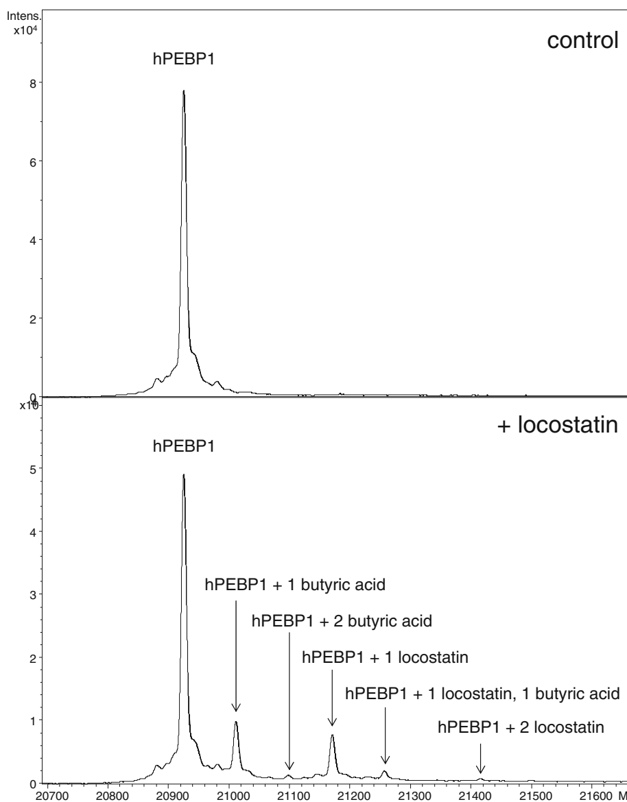
Figure 5. Measurement of TMSF for the hPEBP1-locostatin complex. hPEBP1 and locostatin were incubated for 5 h at 37 °C and excess locostatin removed by micro-gel filtration. The covalent complex was then analyzed by HRMS with online desalting
