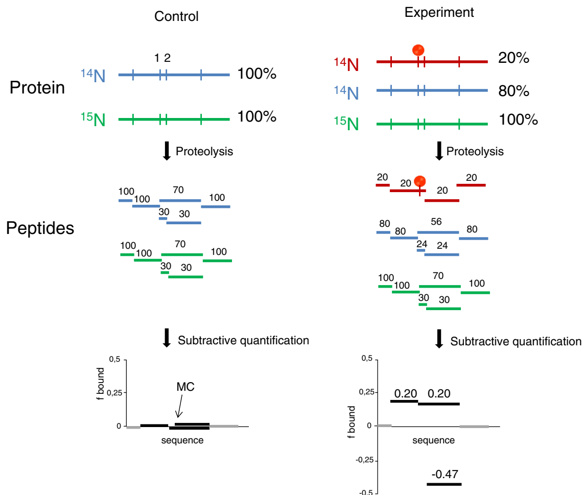
Figure 4. Bound fraction pattern caused by a shifted cleavage. This scheme is valid for both N- and C-endoproteinases. Protein and peptides are represented in color with associated abundances. The corresponding f_{\text{bound}} are calculated using non modified peptides and graphed at the bottom. Two cleavable and modifiable sites separated by two residues are shown: site 1 and site 2. In the control, site 1 is completely cleaved whereas a missed cleavage of 70% is considered at site 2. In the experiment, 20% of ^{14}\text{N} protein is modified at site 1, so that there is a MCm at site 1 and there is no more MC at site 2 in this modified population of protein. The dipeptide generated after cleavages at sites 1 and 2 is not represented in the bottom graphs because of its short length, which impairs its detection by MS
