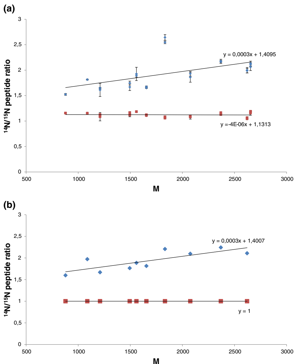
Figure 2. Influence of the number of isotopic distribution peaks used for area calculation on the quantification result. The ^{14}\text{N}/^{15}\text{N} ratios for each peptide were calculated using Skyline software and plotted as a function of M . (a) Asp-N peptides from a 1:1 mixture of ^{14}\text{N}/^{15}\text{N} hPEBP1 protein solutions were analyzed in decaplicate by nanoUltraHPLC-UHR-QTOF MS. (b) Theoretical relative isotopic abundances of the Asp-N peptides of hPEBP1. In blue: the first three peaks of the monoisotopic distribution are considered. In red: The whole monoisotopic distribution (isotope >1%) is considered
