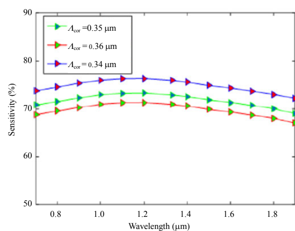
Fig. 5 Variation of sensitivity versus applied wavelength due to tuning the core pitch when other parameters are kept constant.
