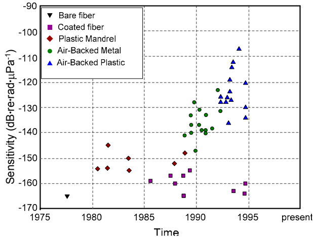
Fig. 8 Progress of interferometric hydrophone system performance in the last 35 years [49].
