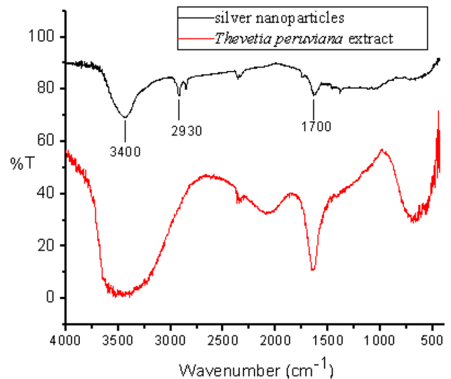
Fig. 5 FTIR spectrum of T. peruviana extract and silver nanoparticles
