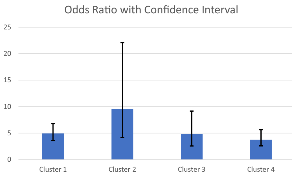
Fig. 3 Visualization of odds ratios with confidence intervals
