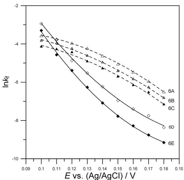
Fig. 5 The dependence of rate constants of 1 \times 10^{-3} \text{ mol dm}^{-3} Bi (III) electroreduction in 6 \text{ mol dm}^{-3} chlorates (VII), where \text{HClO}_4:\text{NaClO}_4 = 1:1 (—) 6A; \text{HClO}_4:\text{NaClO}_4 = 1:4 (—) 6B; \text{HClO}_4:\text{NaClO}_4 = 1:9 (—) 6C; \text{HClO}_4:\text{NaClO}_4 = 4:1 (—) 6D; \text{HClO}_4:\text{NaClO}_4 = 9:1 (—) 6E on the electrode potential
