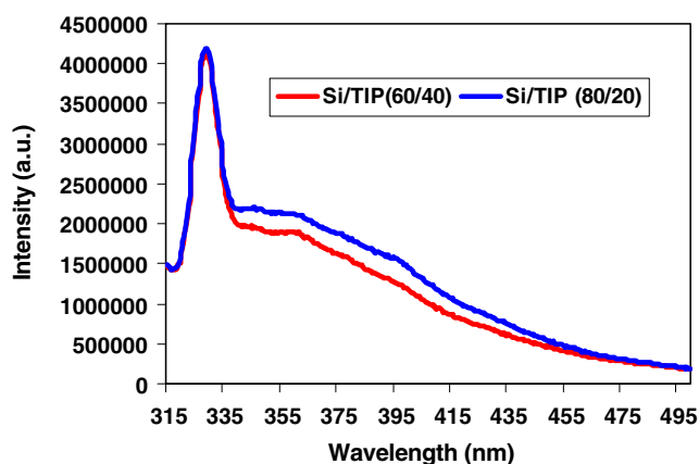
Fig. 11 Photoluminescence (PL) spectra of the Si/TIP system
