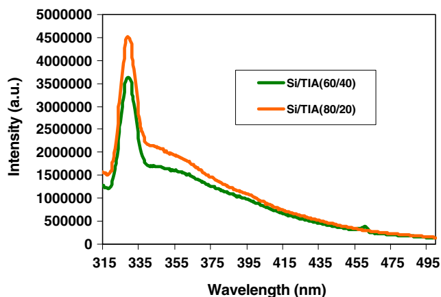
Fig. 12 Photoluminescence (PL) spectra of the Si/TIA system
