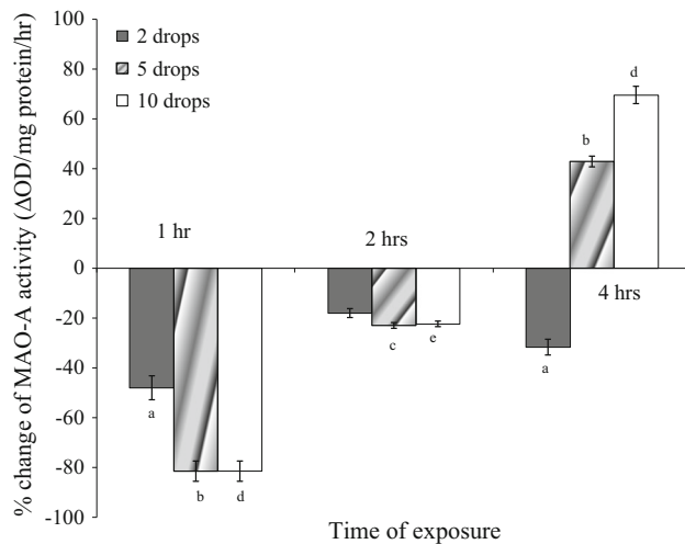
Fig. 3 Blood platelet MAO-A activity (percentage change) in short-term patchouli oil exposure (1, 2, and 4 h) with different dosages (drops) in adult male albino rats. Results (percent change) are expressed as mean \pm SEM of 4–6 separate observations. Each observation was made from a single rat. MAO-A activity was measured using serotonin as a substrate. Patchouli oil exposure was given at different dosages (2, 5, and ten drops). The control value of young rat blood platelet MAO-A activity ( \Delta OD/mg protein/h) is 1.61 \pm 0.033 . Other details are described in the “Materials and methods” section. Significant difference was from control young rats with (i) two drops a p < 0.001 , (ii) five drops b p < 0.001 , c p < 0.01 and (iii) ten drops d p < 0.001 , c p < 0.01
