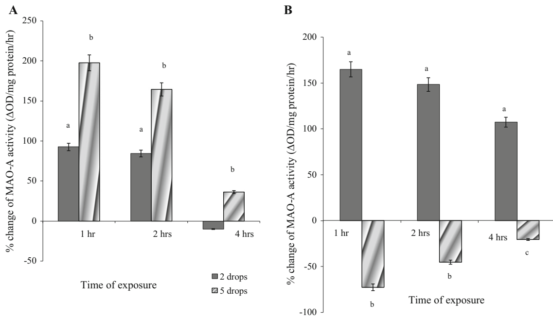
Fig. 5 Blood platelet MAO-A activity (percentage change) in long-term [15 A and 30 B consecutive days] patchouli oil exposure with different dosages (drops) in adult male albino rats. Results (percent change) are expressed as mean ± SEM of 4–6 separate observations. Each observation was made from a single rat. MAO-A activity was measured using serotonin as a substrate. Patchouli oil exposure was given at different dosages (two and five drops). The control value of
