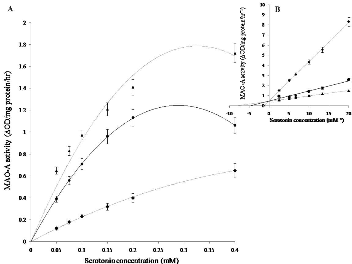
Fig. 4 A Effect of various concentrations of serotonin (0.05–0.4 mM) on blood platelet MAO-A activity in control and short-term single patchouli oil-exposed rats. Results are expressed as mean \pm SEM of 4–6 separate observations. Each observation was made from a single rat. The filled circle represents the control, the filled diamond represents five drops patchouli oil of 1-h single
