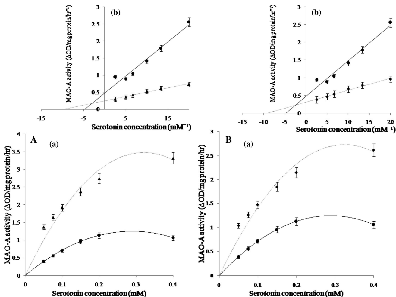
Fig. 6 (a) Effect of various concentrations of serotonin (0.05–0.4 mM) on blood platelet MAO-A activity in control and long-term [A 15 and B 30 consecutive days] patchouli oil-exposed rats. Results are expressed as mean \pm SEM of 4–6 separate observations. Each observation was made from a single rat. The filled circle represents control, the filled triangle represents five drops of patchouli oil of 1-h exposure for 15 consecutive days, the filled
