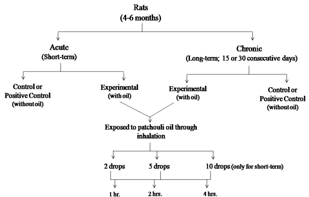
Fig. 2 A schematic diagram of the experimental design
