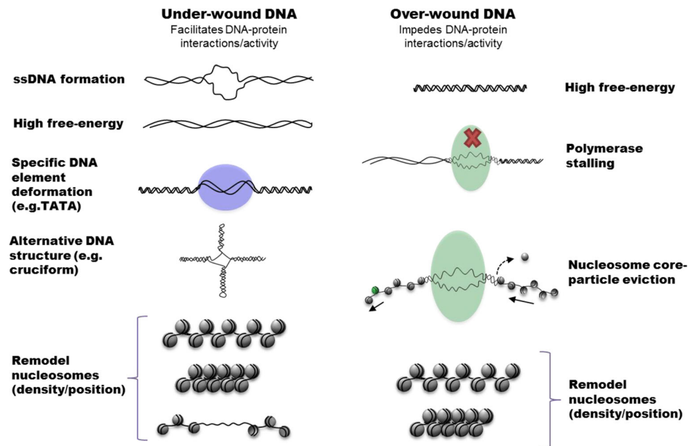
Fig. 4 DNA supercoils influence DNA–protein interactions and catalytic activity. An overview of the ways over- and under- wound DNA can influence DNA structures, protein–DNA interactions and the catalytic activity of DNA binding proteins. ssDNA Single-strand DNA
