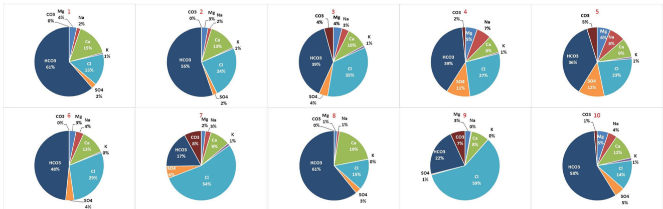
Fig. 5 Pie charts of waters, 1, 2 Dinarsuyu stream, 3 Büyük Menderes River, 4, 5, 6 Kufi stream, 7 Işıklı spring, 8 Yuva spring, 9 Gümüşsu spring, 10 Işıklı Lake
