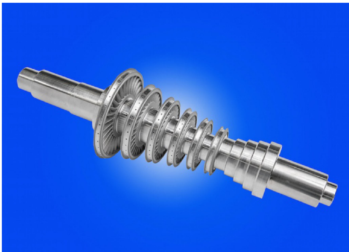
Fig. 2. Additively manufactured rotor for water desalination, roughly 6" (c. 15 cm) in length.
