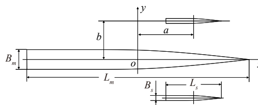
Figure 2 Trimaran configuration
