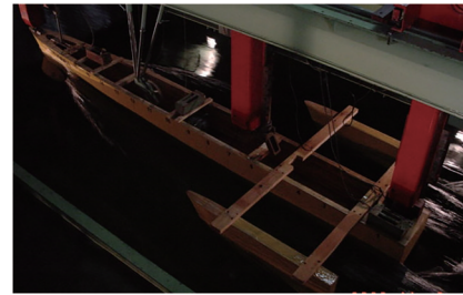
Figure 5 Model tests for Model A in the towing tank
