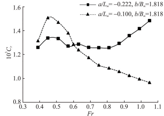
(b) Model C
