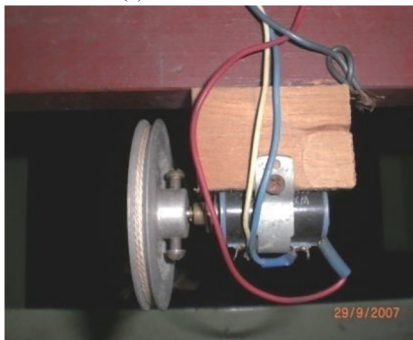
(b) Heaving sensor
