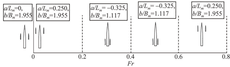
Figure 22 Spectrum of the optimum configuration for the roll and resistance in regular waves
