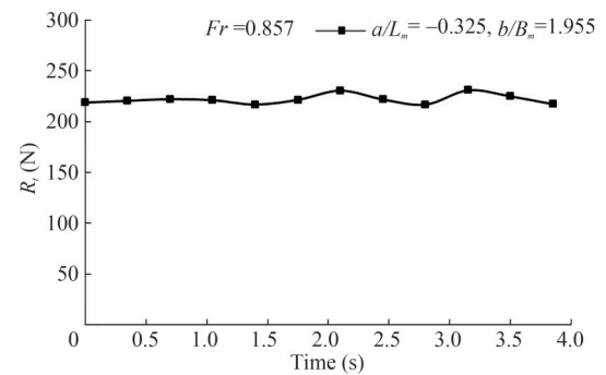
Figure 6 Time history of the total resistance of a/L_m = -0.325 , b/B_m = 1.955 at Fr = 0.857
