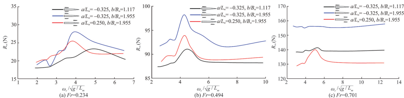
Figure 21 Resistance in waves of different configurations for Model A
