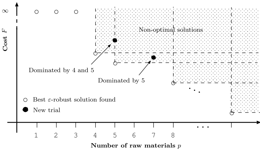
Fig. 2 Pareto optimality
