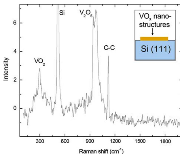
Fig. 8 Raman spectrum of the VO 2 /V 2 O 5 triangular capsules containing VO 2 /V 2 O 5 fullerenes and quantum dots showing a strong peak at 1,120 cm -1 which suggests C–C intercalation of the VO 2 /V 2 O 5 structure
