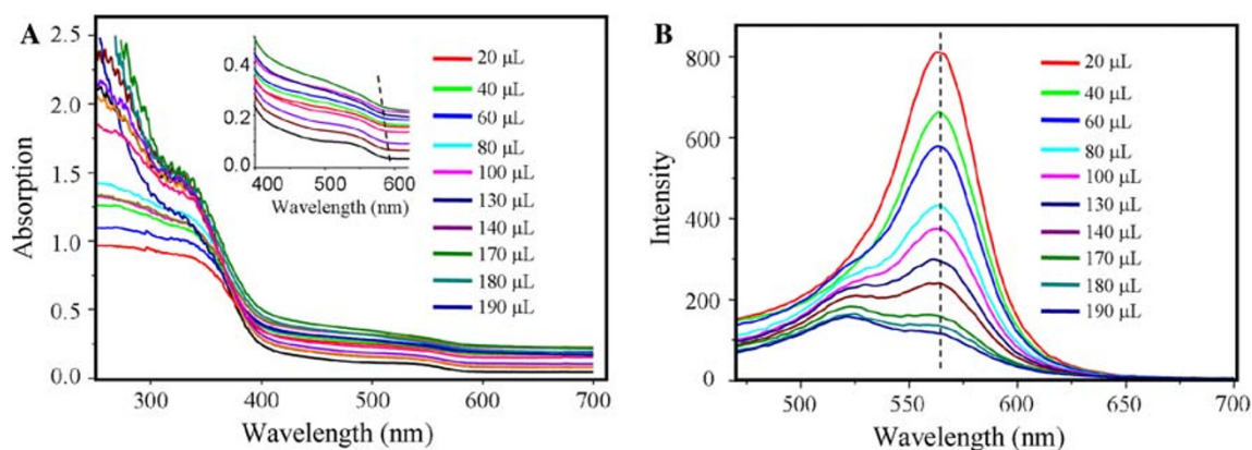
Fig. 4 The UV-vis absorption (a) and photoluminescence spectra (under excitation at 400 nm) (b) of CdSe QDs upon addition of AO/CNTs. The insert of (a) shows the slight blue shift of the CdSe absorption edge during titration
