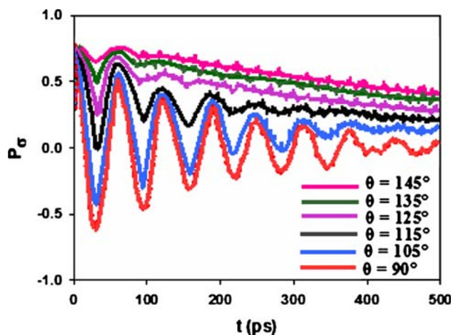
Fig. 1 Variation of P_\sigma with the orientation ( \theta ) of the magnetic field
